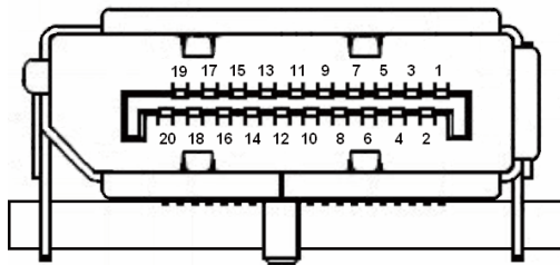
20-pin color display signal cable
